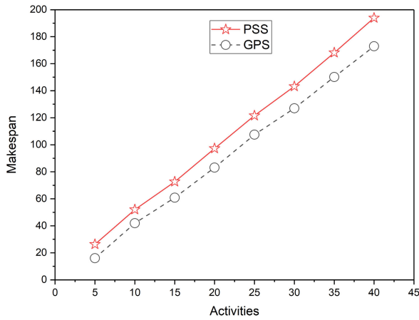
FIGURE 4. Experiment 2: Impact of number of tasks on project makespan.
