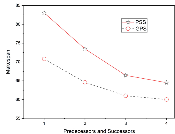
FIGURE 7. Experiment 5: Impact of graph complexity.
